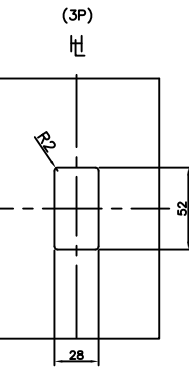
盤面孔面 Panel Cutout
