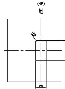
盤面孔面 Panel Cutout
