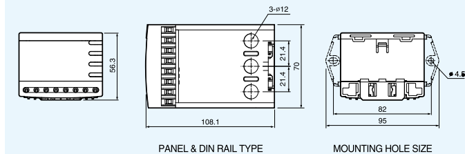
EOCR-3DM2-HZ(過孔式)
