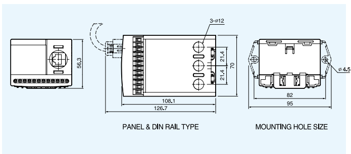
EOCR-iFDM-HZ / iFM420-HZ (過孔式)
