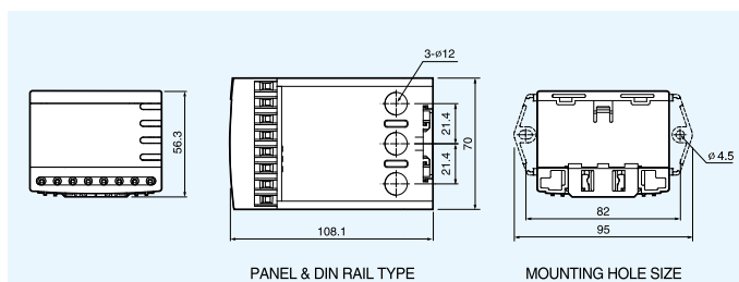
EOCR-3DM2-HZ(過孔式)
