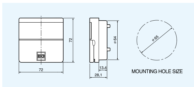
EOCR-PDM (Display)
