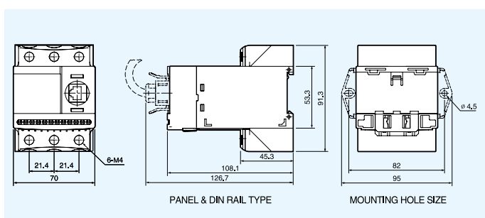
EOCR-iFDM-TZ / iFM420-TZ (端子式)
