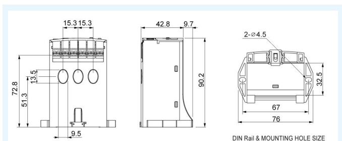
EOCR-SE2
