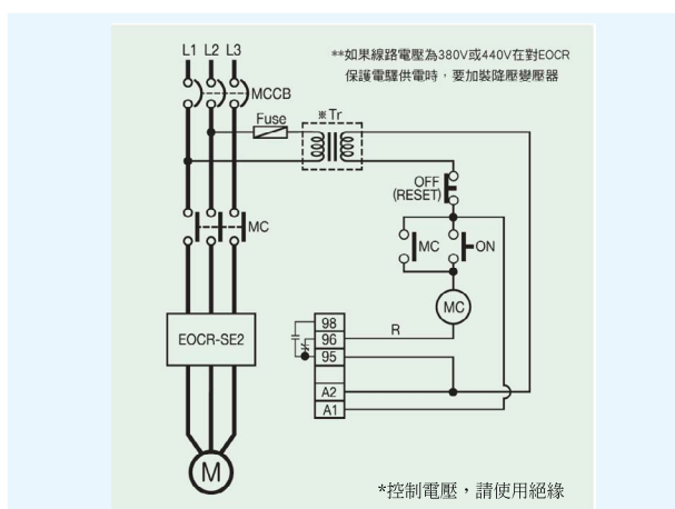
EOCR-SE2
