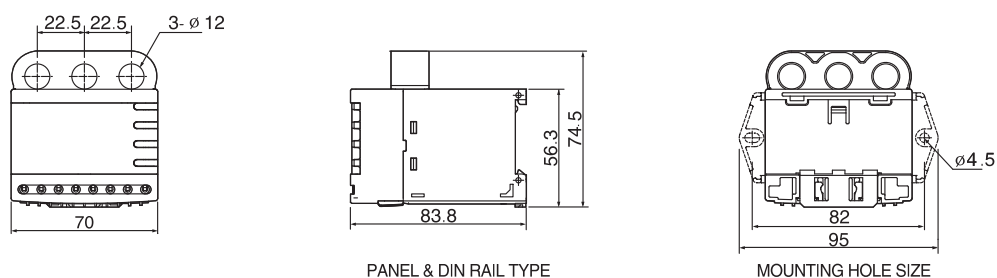
PANEL &amp; DIN RAIL TYPE
