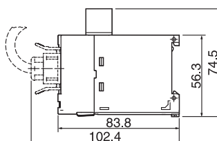
PANEL &amp; DIN RAIL TYPE
