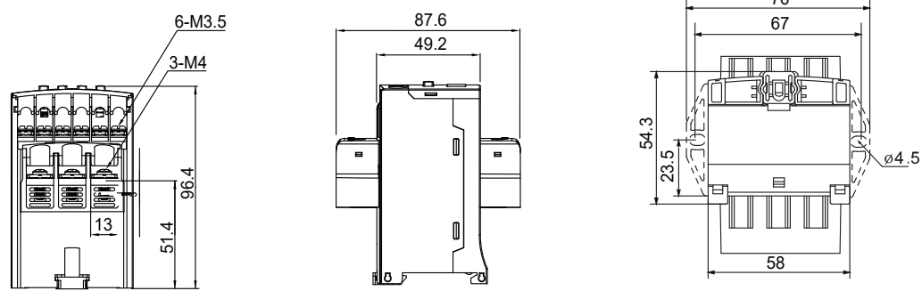
MOUNTING HOLE SIZE
