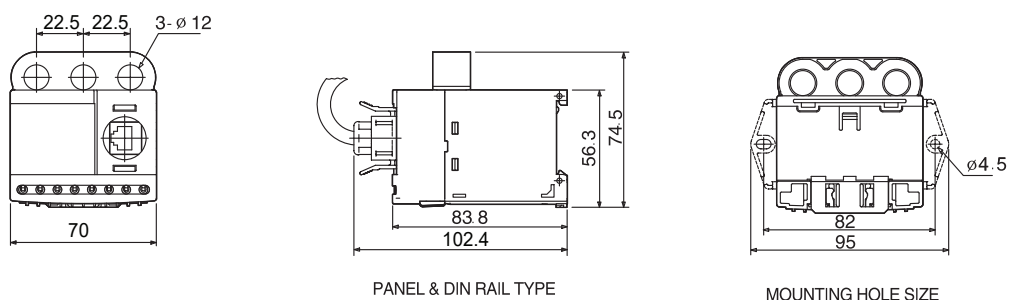
MOUNTING HOLE SIZE
