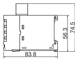
PANEL &amp; DIN RAIL TYPE
