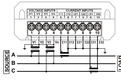
3P3W-2PT/2CT[設定:3P3Y]
