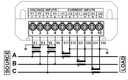
3P3W-2PT/3CT[設定:3P3Y3]
