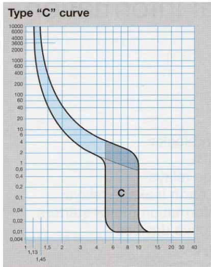
Characteristic curve
