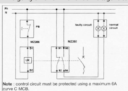
Emergency swith-off with under-voltage release
