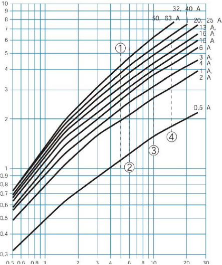
Characteristic curve
