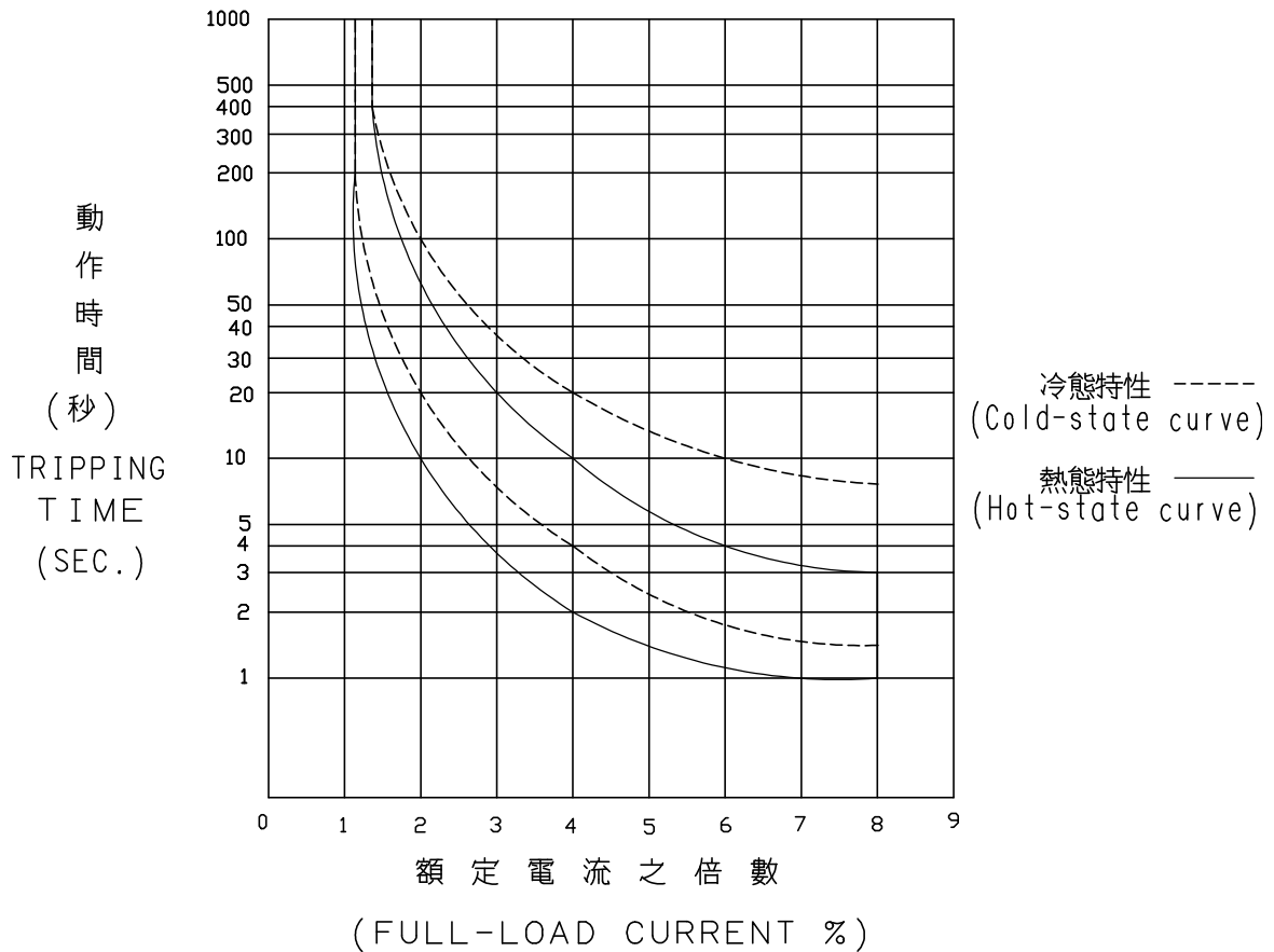
三相健全時之動作時間特性 (three-phase overcurrent characteristics)
