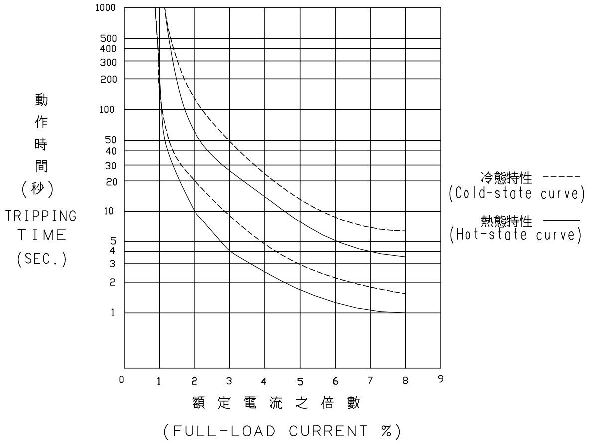
欠相時之動作時間特性 (single-phase protection characteristics)
